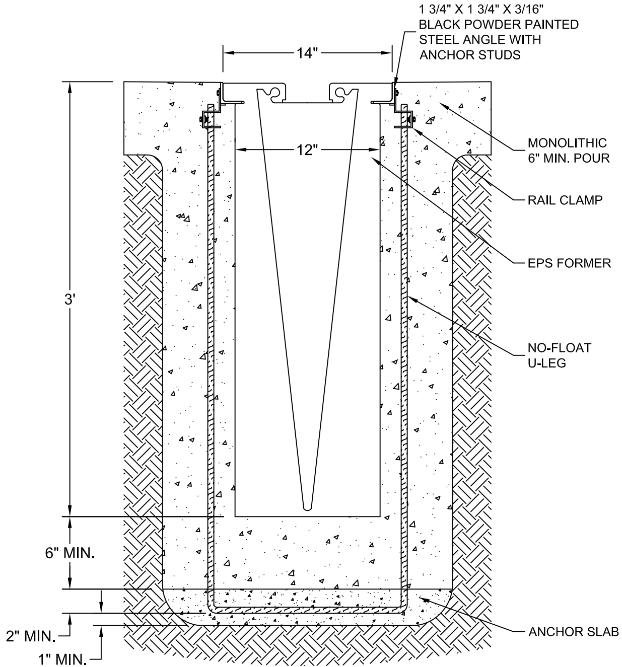
END CROSS SECTION VIEW
