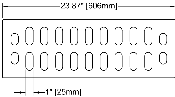
GRATE TOP VIEW (ROTATED 90°)
