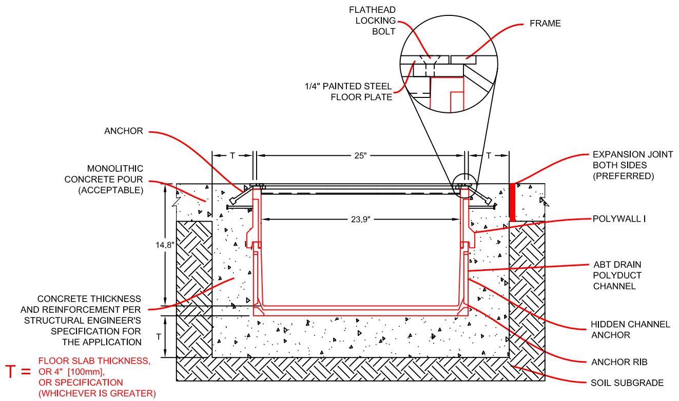
CROSS SECTIONAL VIEW
