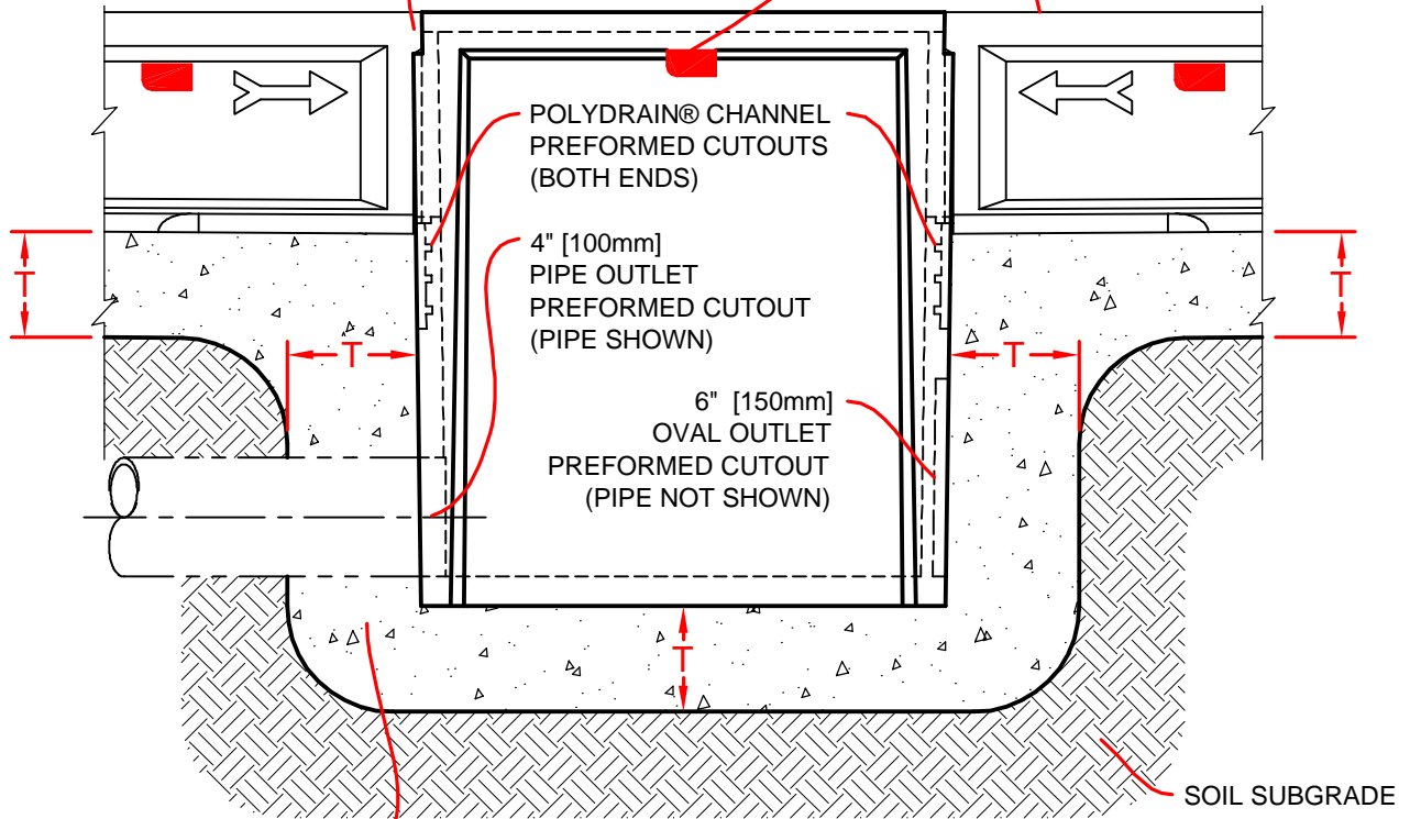
ELEVATION VIEW
