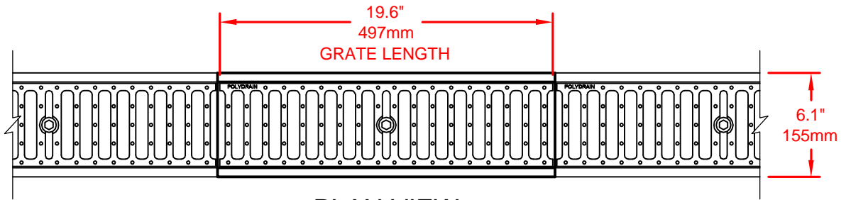
PLAN VIEW
