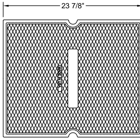
PLAN VIEW #1500.20 C.I. COVER
