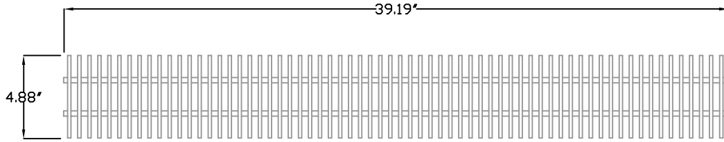
#2722 FRP GRATE (FIBERGLASS) (1/4" BARS @ 5/8" O.C.)
