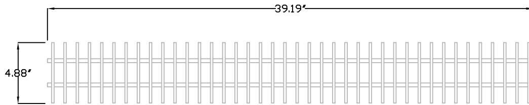
#2720 FRP GRATE (FIBERGLASS) (1/4" BARS @ 1" O.C.)
