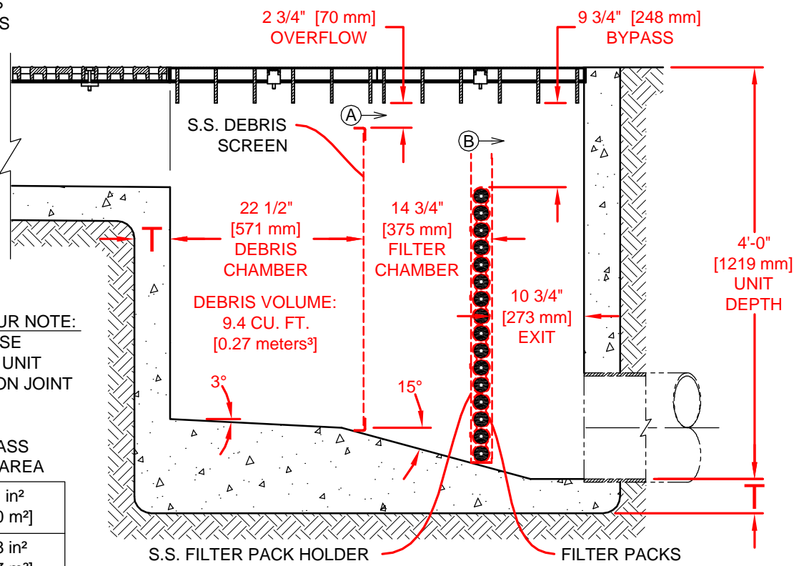
CROSS SECTIONAL VIEW
