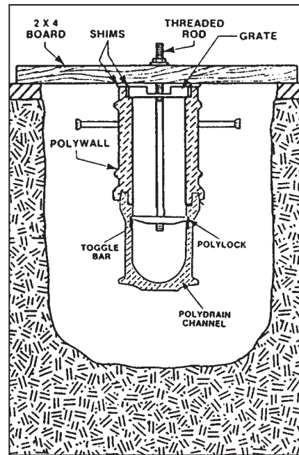
Suspended method with PolyWall Sidewall extensions
