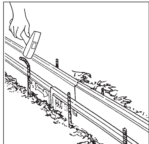
With the first pour set and PolyWing Hangers detached, bend top of rebar over or cut of below finished grade
