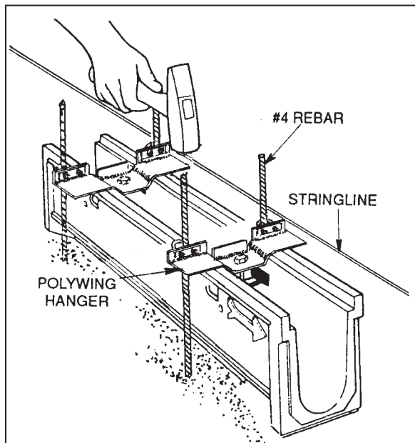
Driving rebar through PolyWing clamps
