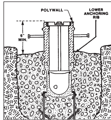
Concrete placed above lower anchoring rib of PolyWall
