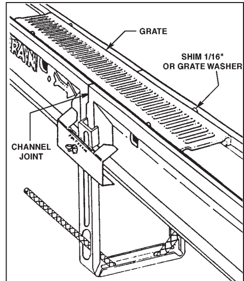
Placement of grate across channel joints
