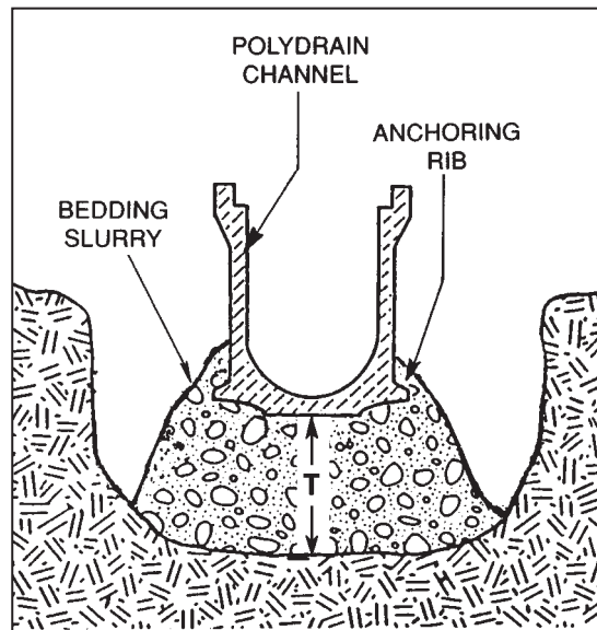
Placement of channel in concrete bedding slurry T = thickness of slab design
