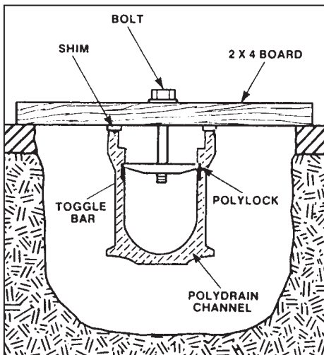
End view of suspended channel installation
