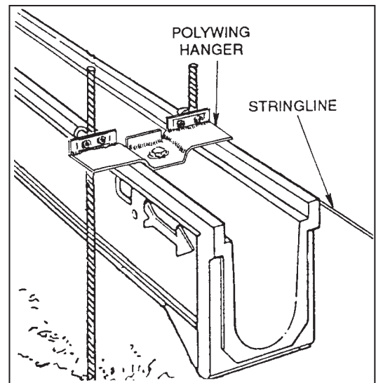
Slide channels with PolyWing Hangers up the rebar until channels are properly aligned with the stringline
