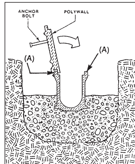
End view of PolyWall placement on channel
