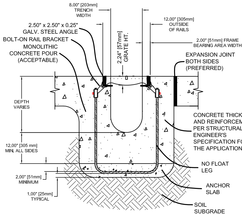
END CROSS SECTION VIEW
