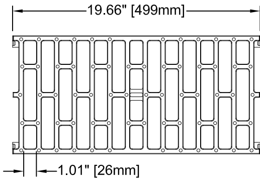
GRATE TOP VIEW (ROTATED 90°)
