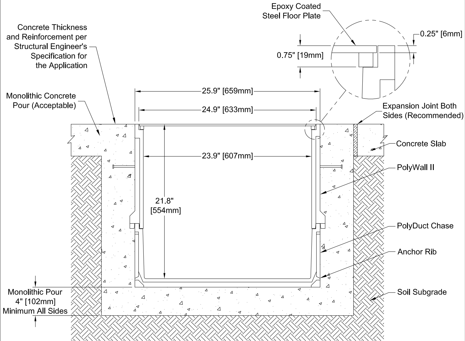
END CROSS SECTION VIEW
