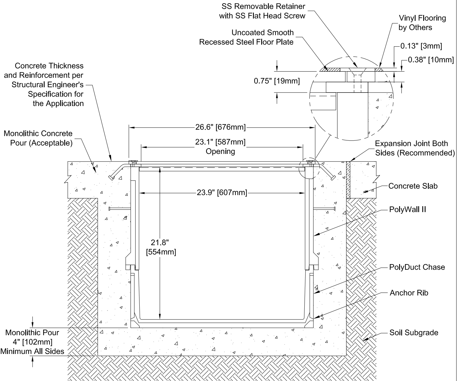
END CROSS SECTION VIEW
