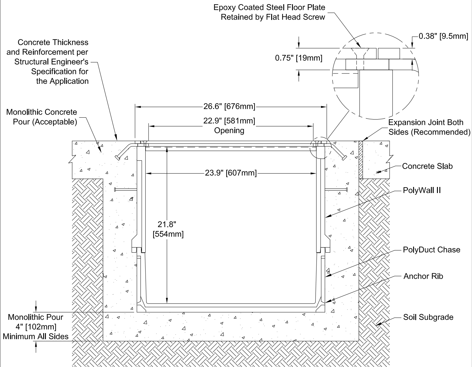
END CROSS SECTION VIEW
