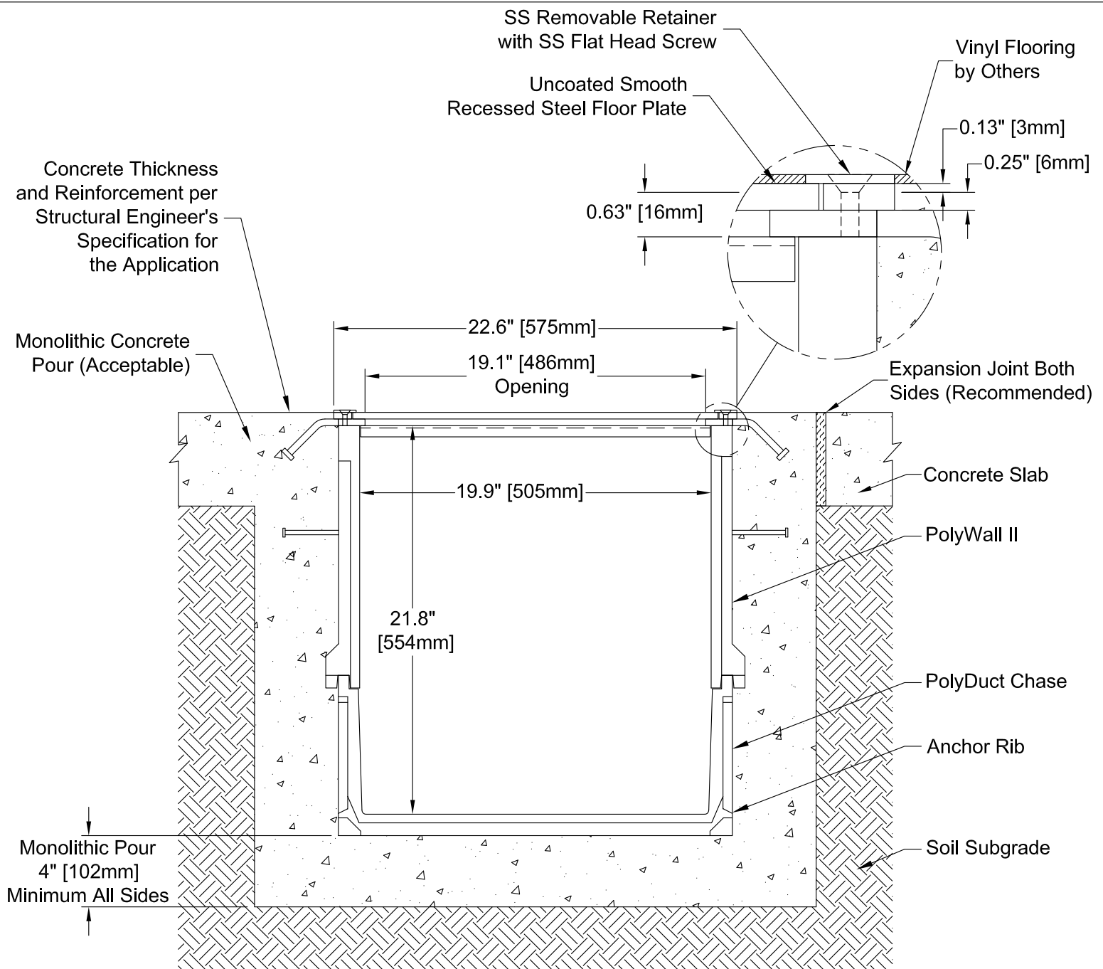
END CROSS SECTION VIEW
