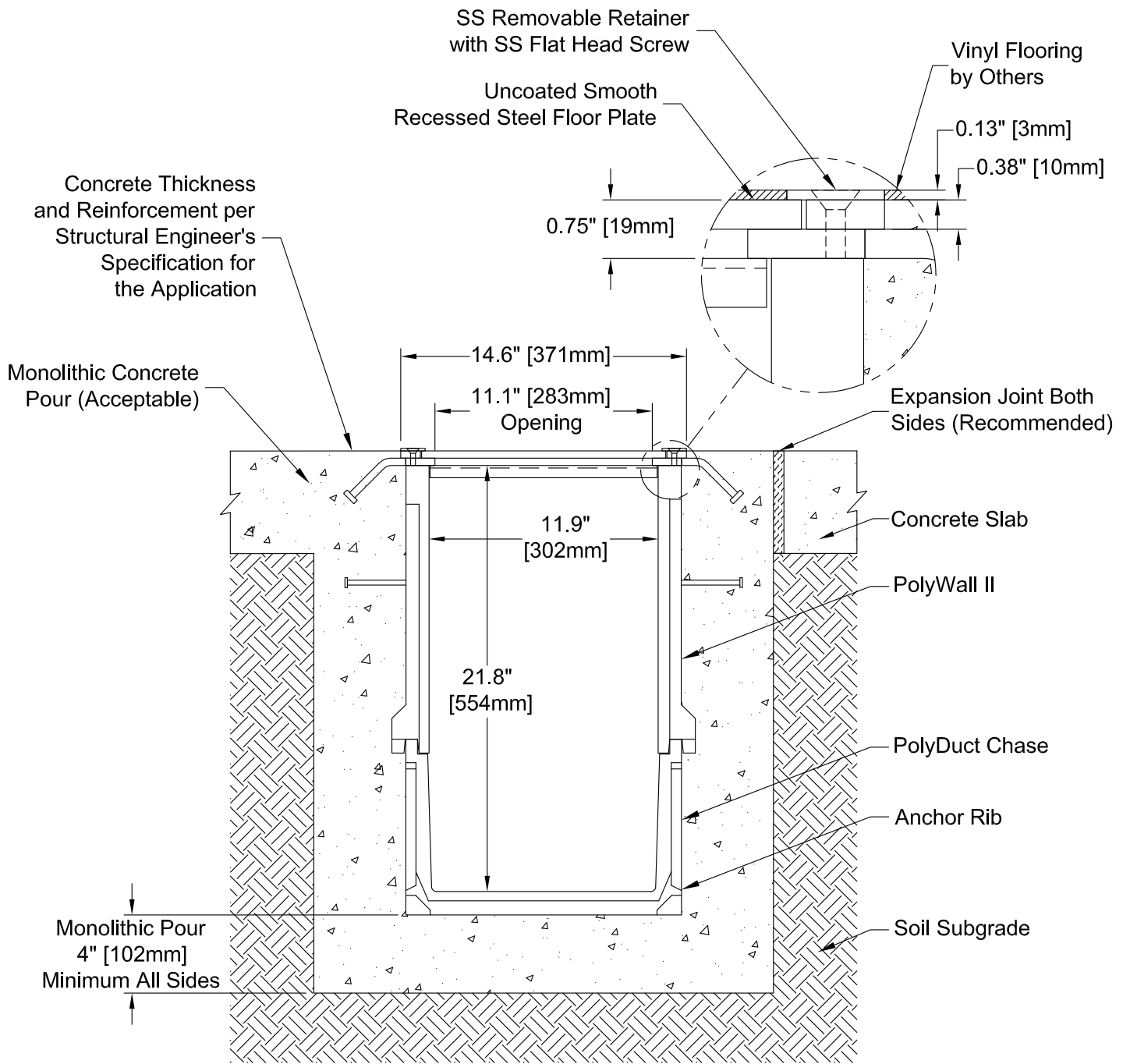
END CROSS SECTION VIEW
