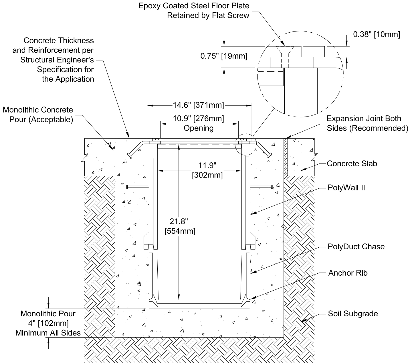
END CROSS SECTION VIEW
